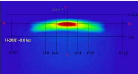
Additional Reflector
